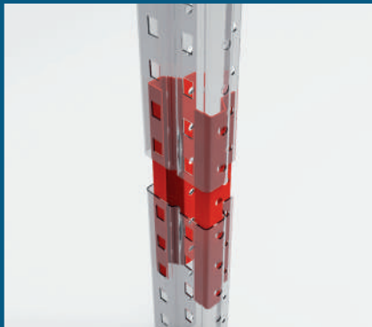
Upright Splice
